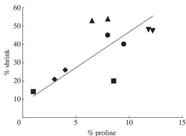
Figure 2. Relationship, showing standard regression curve, between the % shrink and % proline (used to represent MaSp2 compositions in the regression model) of 'ground state' (supercontracted) silks using data for all 10 species examined combined. Each point represents a mean value obtained for six individuals of one species. Triangles, Cyclosa spp.; squares, Nephila spp.; diamonds, Cyrtophora spp.; circles, Argiope spp.; inverted triangles, Leucauge spp.
